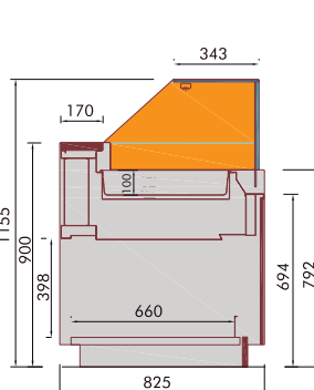
Bellini Lux BM VVRB
