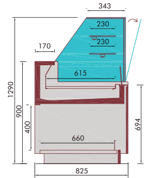
Bellini FV VVR S/R Bellini N VVR S/R Bellini CH VVR S/R
