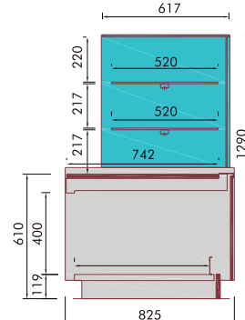
Bellini Torre N
