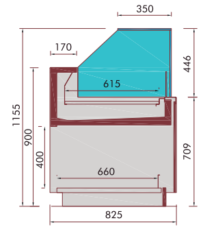
Bellini FV VC S/R Bellini N VC S/R Bellini CH CV S/R
