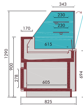
Bellini FV VVR C/R
