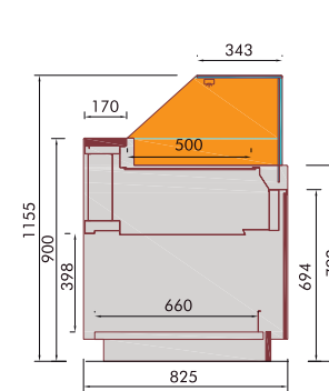
Bellini PQ VVRB
