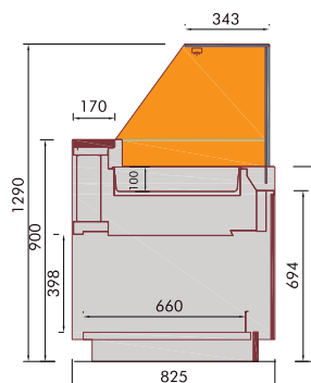
Bellini BM VVR
