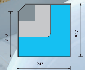
Bellini VVR S/R EXT 90°
