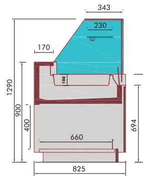
Bellini CR VVR
