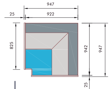
Bellini VVR S/R INT 90°
