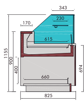
Bellini FV VVRB S/R Bellini N VVRB S/R Bellini CH VVRB S/R
