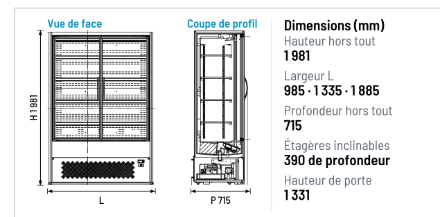
COUPE TECHNIQUE (MM)
